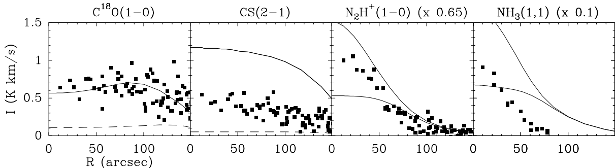
FIG. 7.— Comparison between L1517B observations (solid squares) and expected emission from Bergin & Langer (1997) models (lines). In the C^{18}O and CS panels, the dashed lines correspond to the BM94 model (their Model 1), and the solid lines indicate the accretion model (Model 2). In the N_2H^+ and NH_3 panels, only results for the accretion model are shown. The top lines in these panels represent no depletion, and the bottom lines represent a factor of 10 depletion for densities higher than those studied by Bergin & Langer (1997) (see text). All models assume dust grains with H_2O mantles, and to simplify the display, both model and data in the two rightmost panels have been scaled down by 0.65 ( N_2H^+ ) and 0.1 ( NH_3 ).
